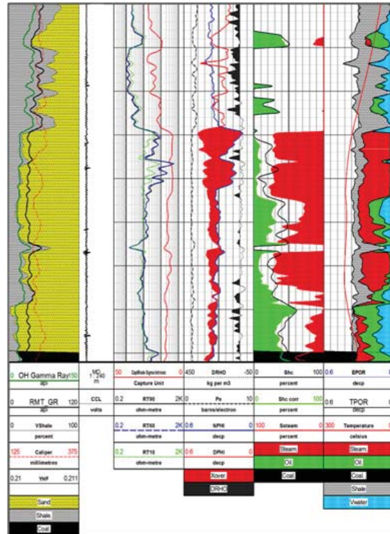
Processed pulsed-neutron data in steam flood:
