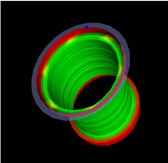
This 3D view from WIPER software shows the variation in ID after setting Casing Patch.
